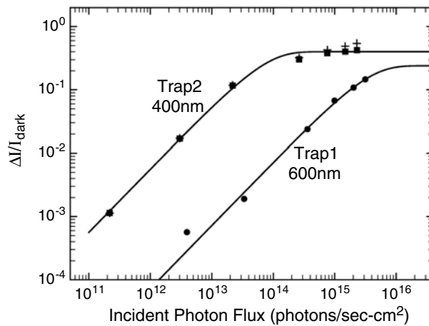
Figure 7. Photoionization saturation measurements in a GaN MESFET for a 5 s illumination time. The filled circles are experimental data taken at 600 nm (only Trap1 photoionized) and the + symbols are for 400 nm data (both traps photoionized). The squares indicate the Trap2 contribution to the latter. The full curves are fits to the data using equation (12).
